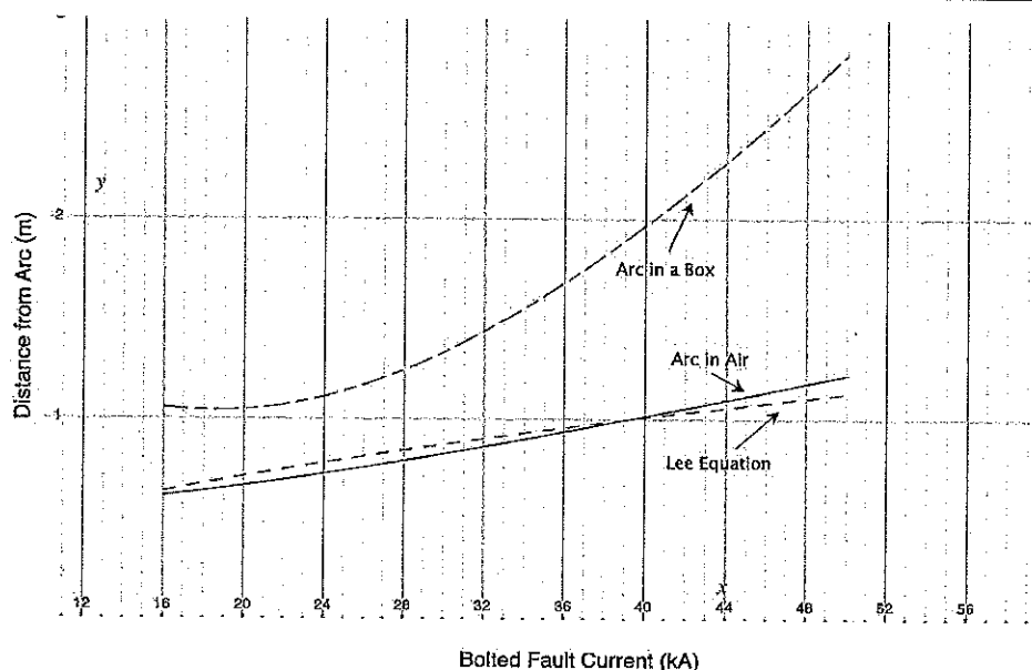
Figure 8--Curable Burn Distance
