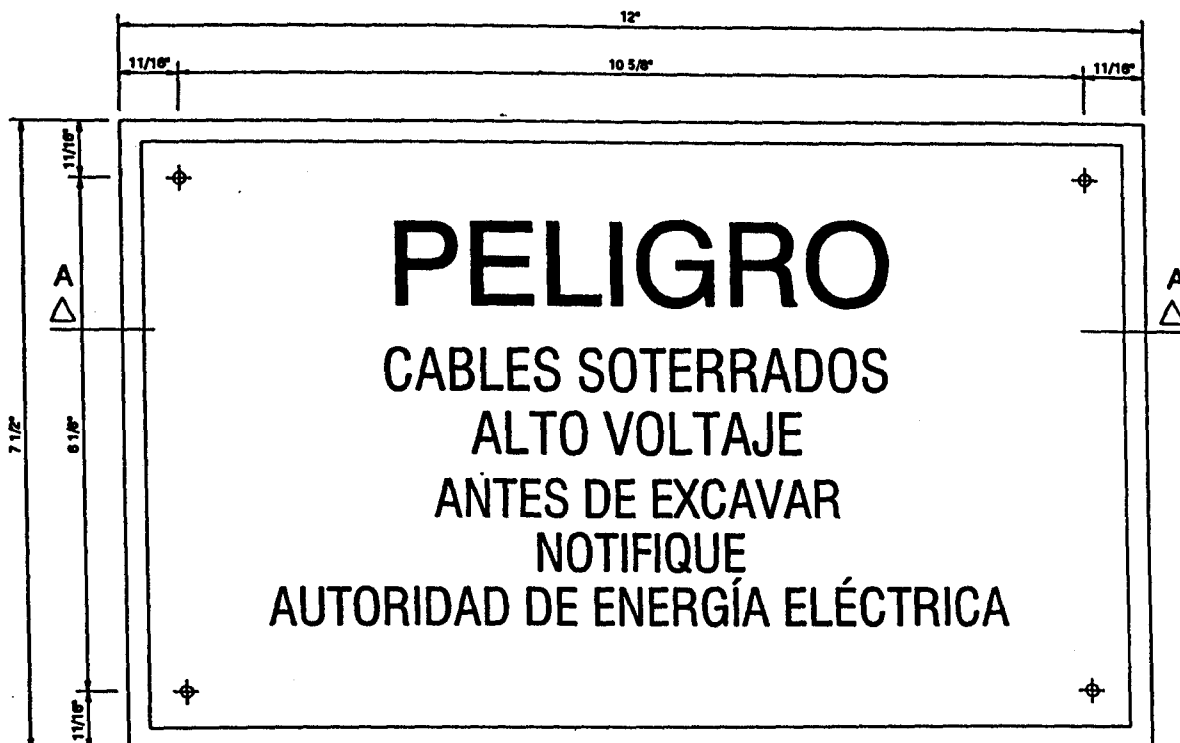
VISTA FRONTAL
