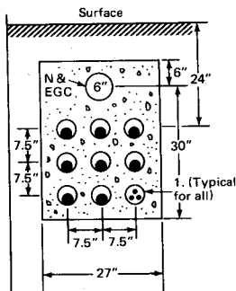
Figure B-310-3. Ampacities of Single Insulated Conductors Rated 0 through 5000 Volts in Underground Electrical Ducts (Three Conductors per Electrical Duct) Nine Single-Conductor Cables per Phase Based on Ambient Earth Temperature of 20°C (68°F), Conductor Temperature 75°C (167°F)
