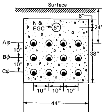
Figure B-310-4. Ampacities of Single Insulated Conductors Rated 0 through 5000 Volts in Nonmagnetic Underground Electrical Ducts (One Conductor per Electrical Duct) Four Single-Conductor Cables per Phase Based on Ambient Earth Temperature of 20°C (68°F), Conductor Temperature 75°C (167°F)
