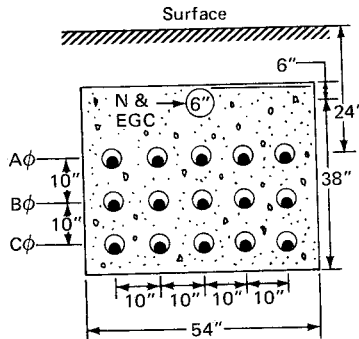
Figure B-310-5. Ampacities of Single Insulated Conductors Rated 0 through 5000 Volts in Nonmagnetic Underground Electrical Ducts (One Conductor per Electrical Duct) Five Single-Conductor Cables per Phase Based on Ambient Earth Temperature of 20°C (68°F), Conductor Temperature 75°C (167°F)
