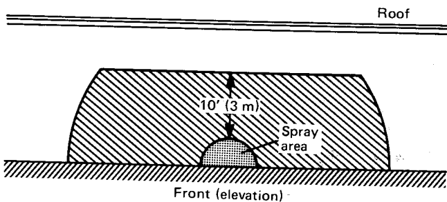
Figure 1. x Class I or Class II, Division 2 Location Adjacent to an Unenclosed Spray Operation.
