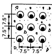
Detail 4 27"x27" Electrical duct bank Nine electrical ducts
