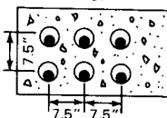
27"x19" Electrical duct bank Six electrical ducts
