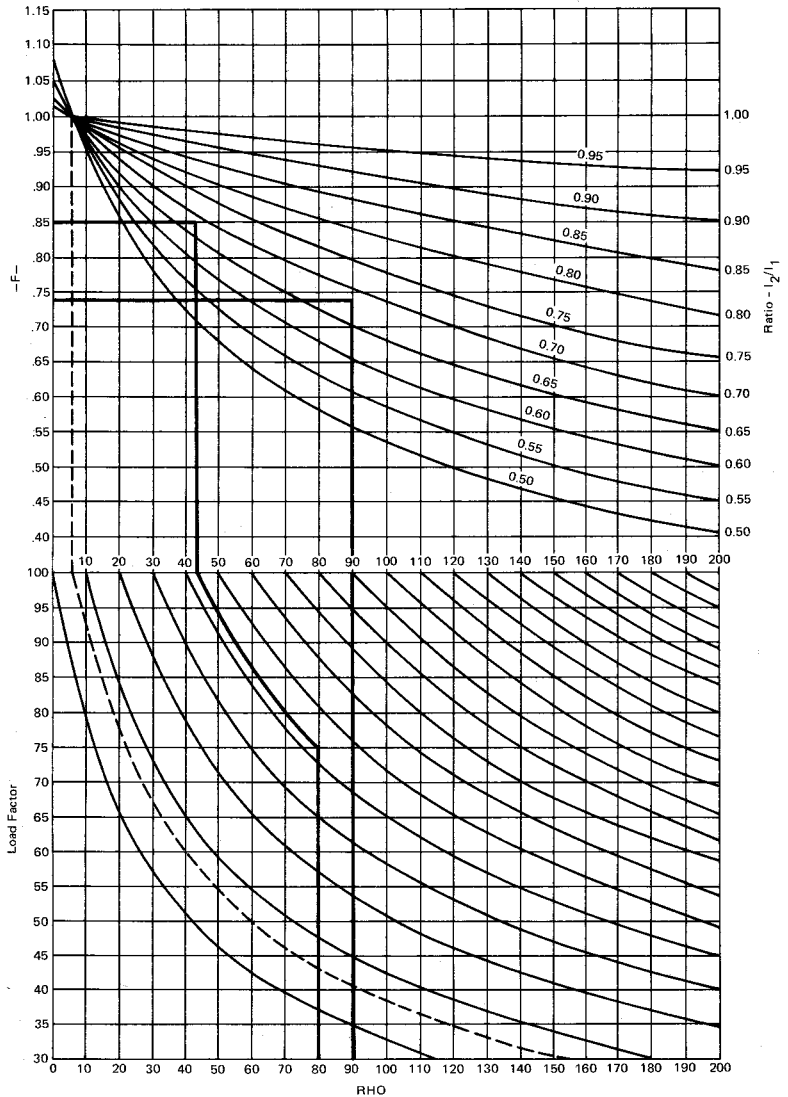
Figure B-310-1. Interpolation Chart for Cables in a Duct Bank I_1 = Ampacity for Rho - 60, 50 LF; I_2 = Ampacity for Rho-120, 100 LF; Desired Ampacity = F \times I_1
