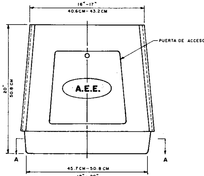
VISTA FRONTAL
